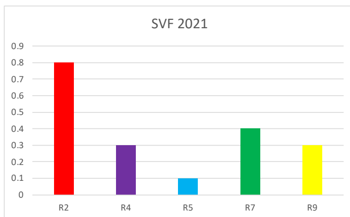
Figure 3. Sky View Factor (SVF) values at receptor points R2, R4, R5, R7, and R9 in Furn Hayek (2021).
