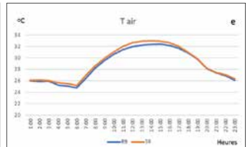
Figure 7. Composite layout of hourly air temperature variations at multiple receptors (2010 vs. 2021), highlighting local microclimatic differences due to SVF and urban geometry in Furn Hayek in 11 august.
