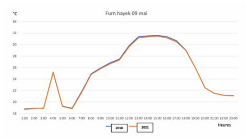
Figure 1. Hourly air temperature variation in Furn Hayek on May 9 for 2010 and 2021 based on ENVI-met simulations.
