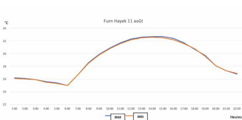
Figure 2. Hourly air temperature variation in Furn Hayek on August 11 for 2010 and 2021 based on ENVI-met simulations.
