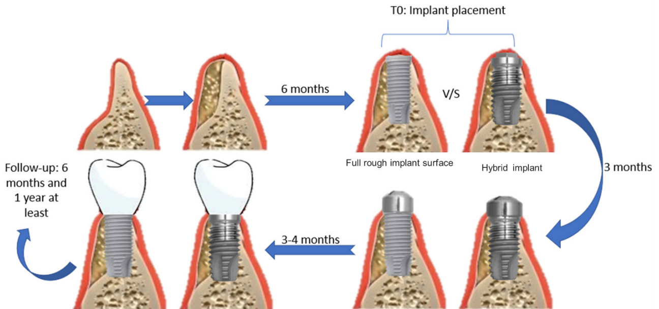
Figure 1: Study Timeline.
